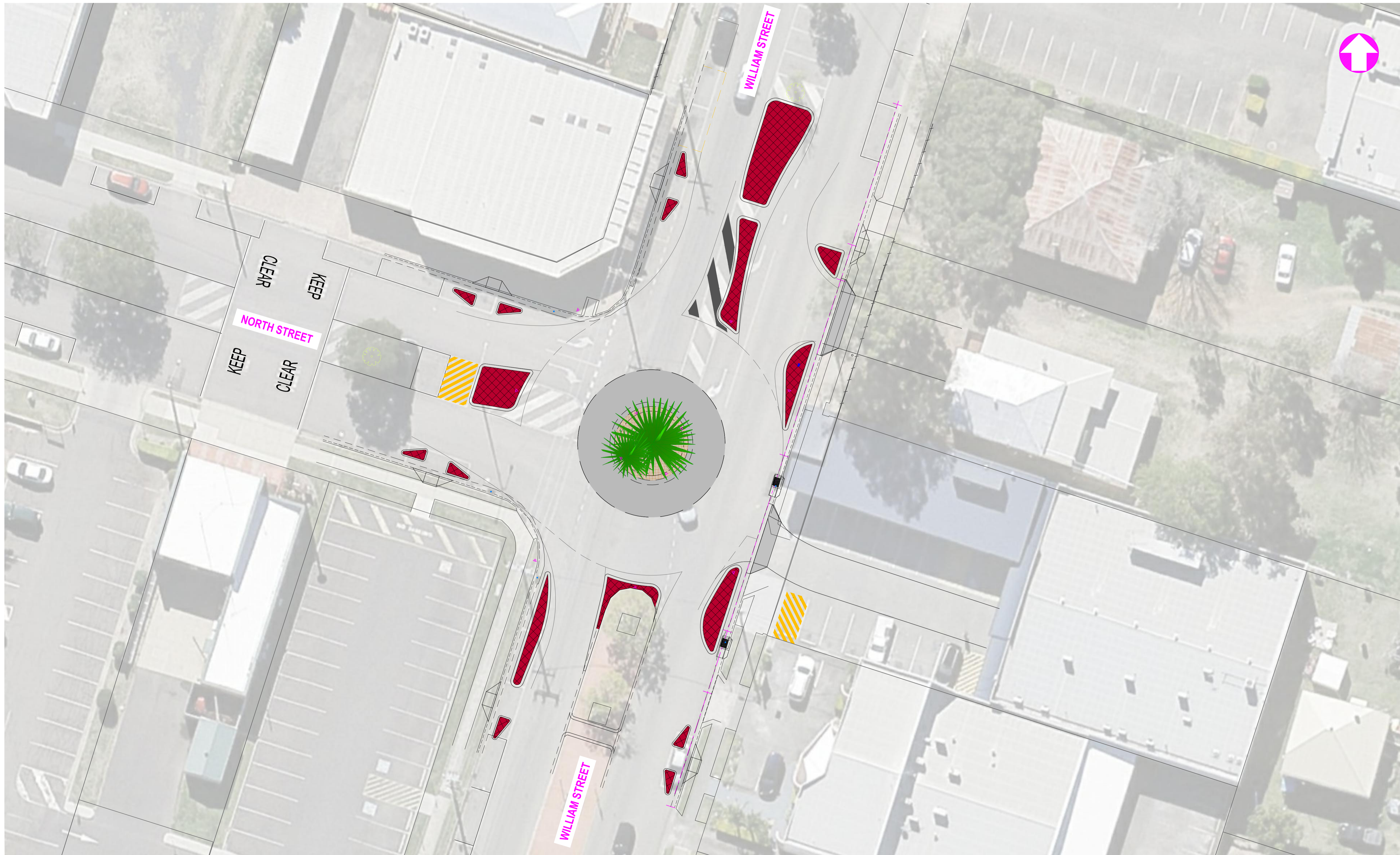
LAYOUT PLAN SCALE 1:200
